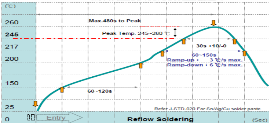
IR Reflow soldering.
